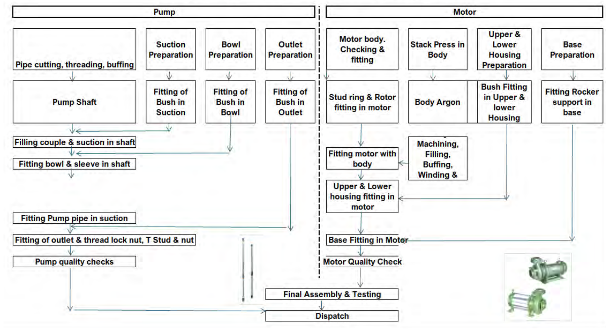
Manufacturing process of a typical stage submersible pump [V-3, 1 Hp]
