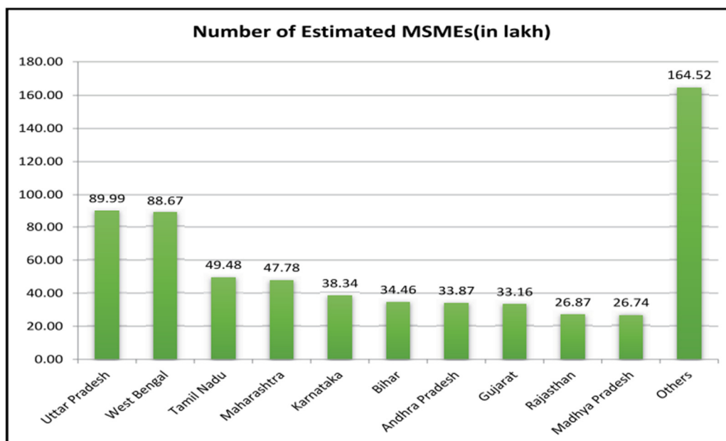
Figure 2.8: Distribution of MSMEs in Top Ten States
